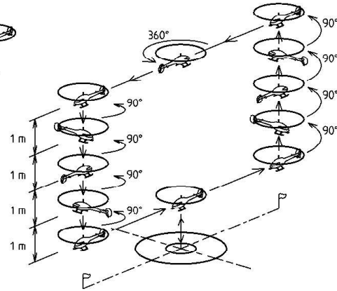
3. RECTANGLE WITH 4-POINT PIRQUETTES
